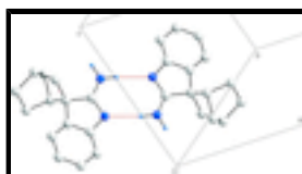
Fig. 2. Packing diagram of (I). Intermolecular N—H...N hydrogen bonds are shown as dashed red lines forming dimers. Note that the anti H2 is not used in any hydrogen bonding interactions.
